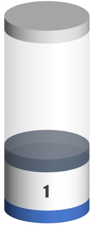
LSO Formation
